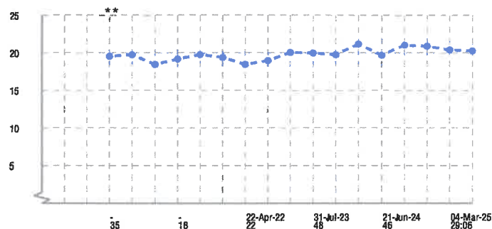
Viscosity at 100°C (cSt | mm2/s)
