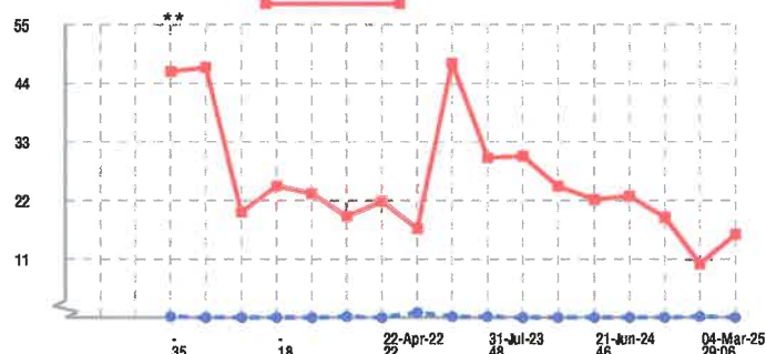
Iron (ppm (wt))
